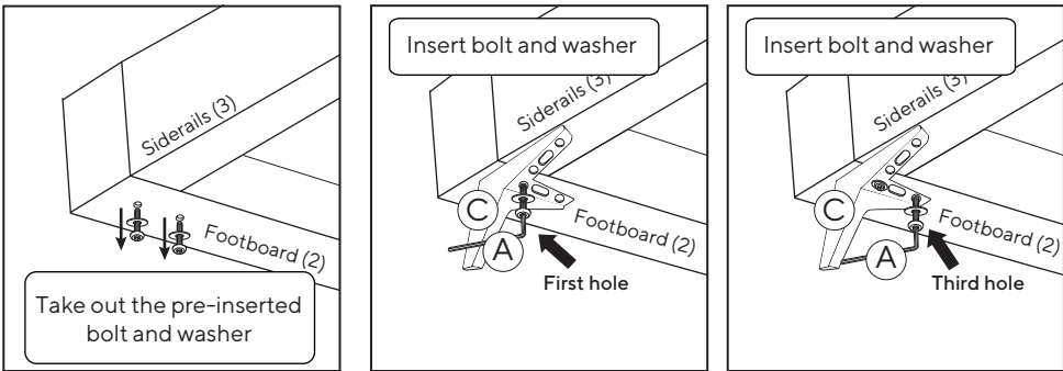
Footboard (2)
