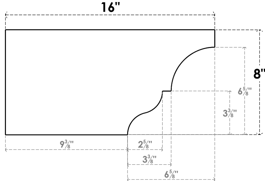
SIDE PROFILE
