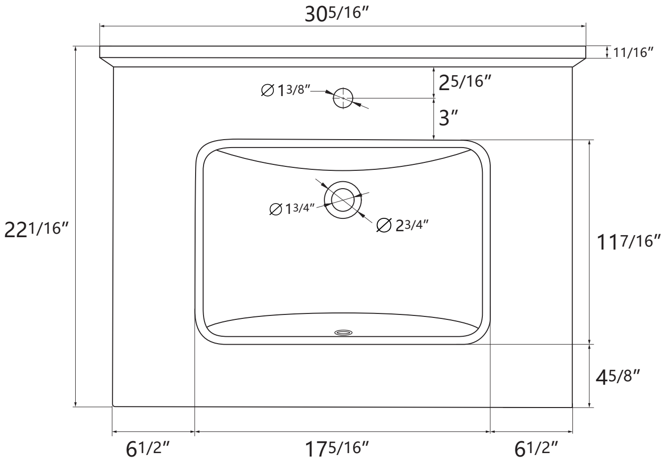
Top View
