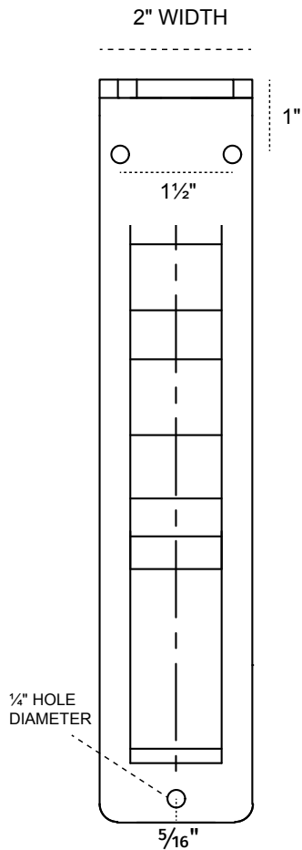
FRONT PROFILE
