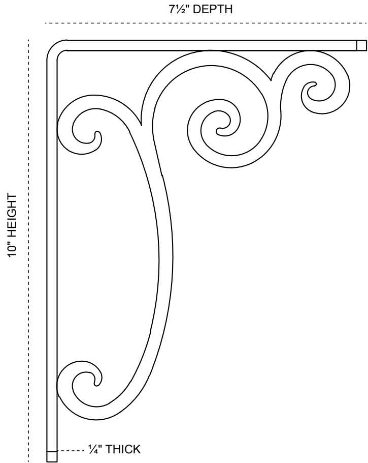
SIDE PROFILE
