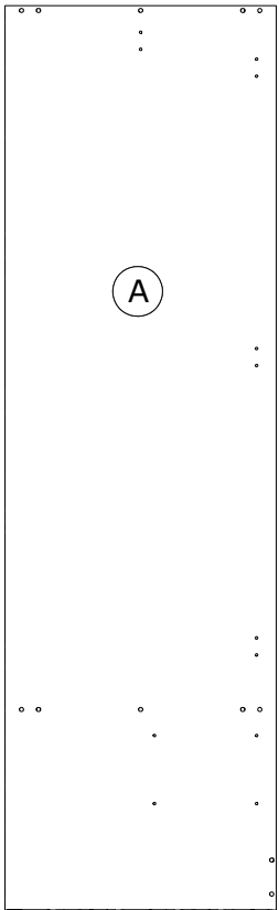
FI2846 1700x510x16mm
