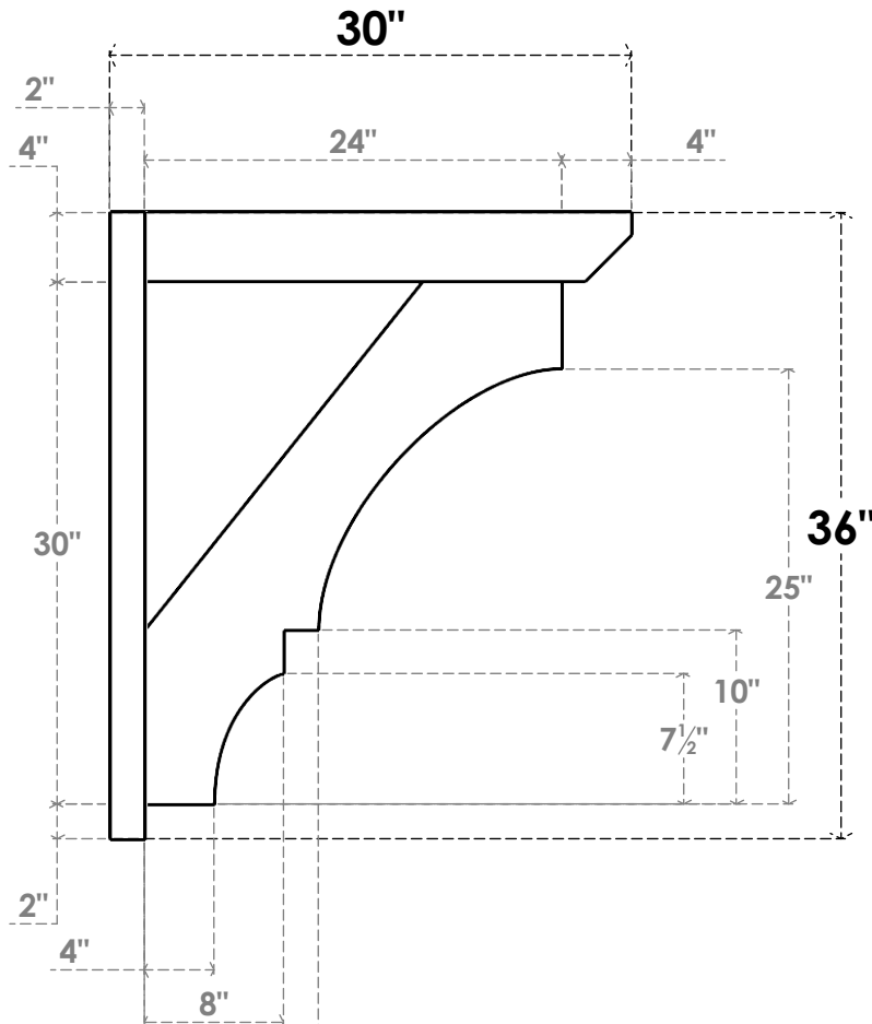
SIDE PROFILE
