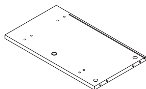
9 (582*164*15mm x1)
