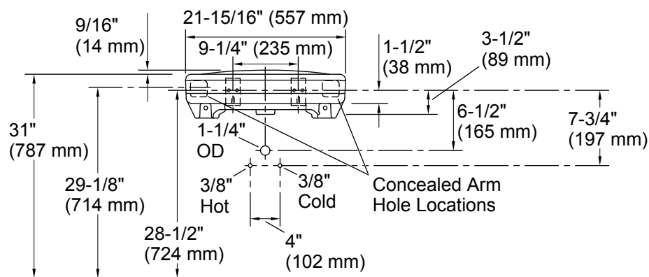
Standard Installation
