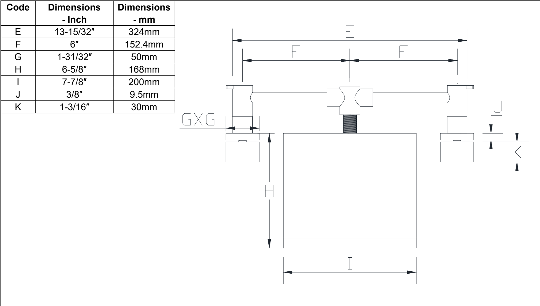
TOP VIEW OF FAUCET
