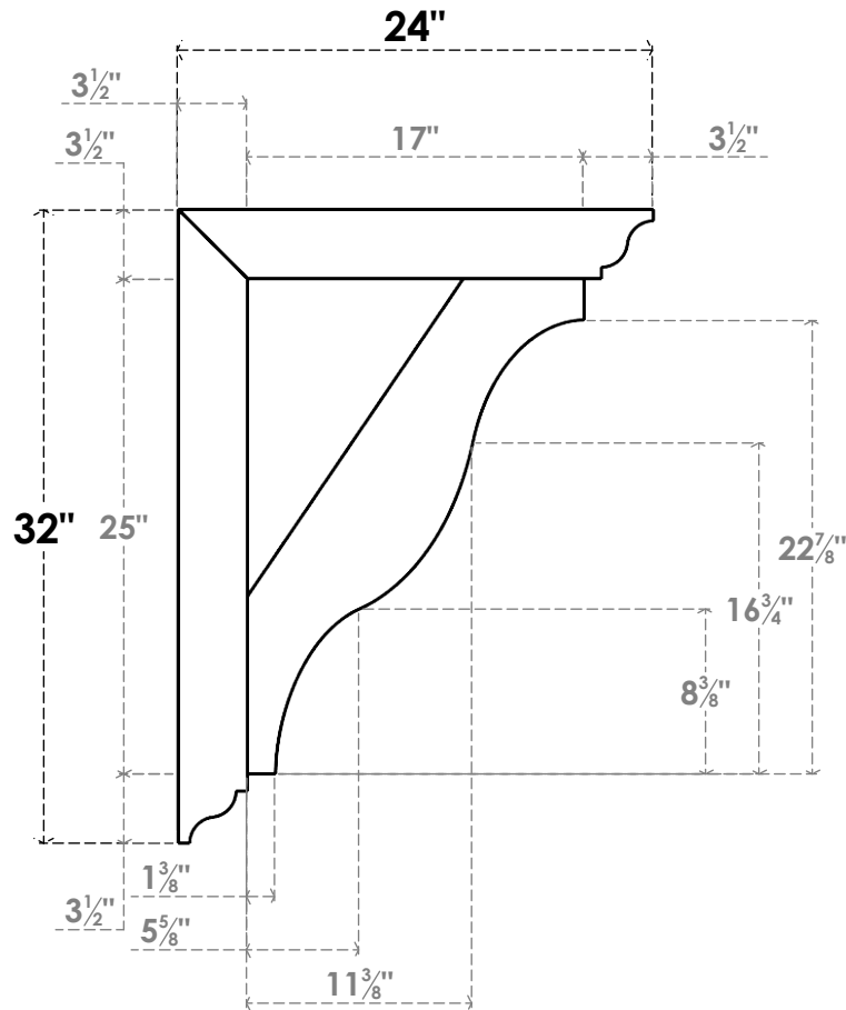
SIDE PROFILE
