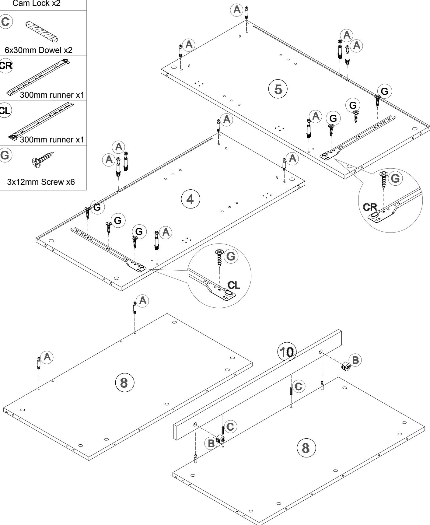
Cam Lock x2
