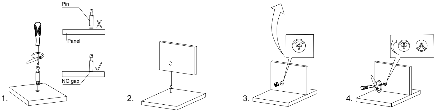
Connecting piece
