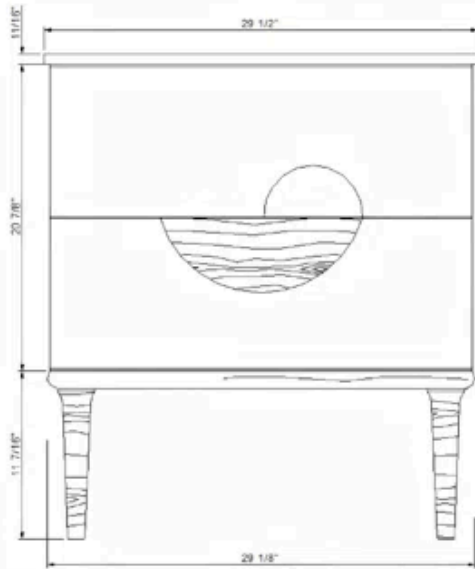
Elevation view
