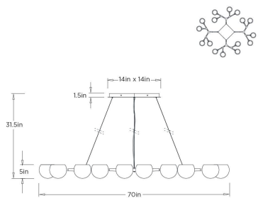
DLC53 MAHOWALD FIXED CHANDELIER
