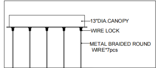
CANOPY DETAIL
