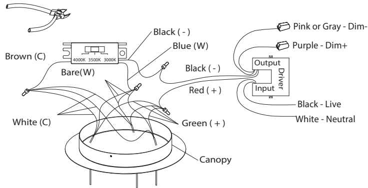
Fig. 4 Wire Diagram
