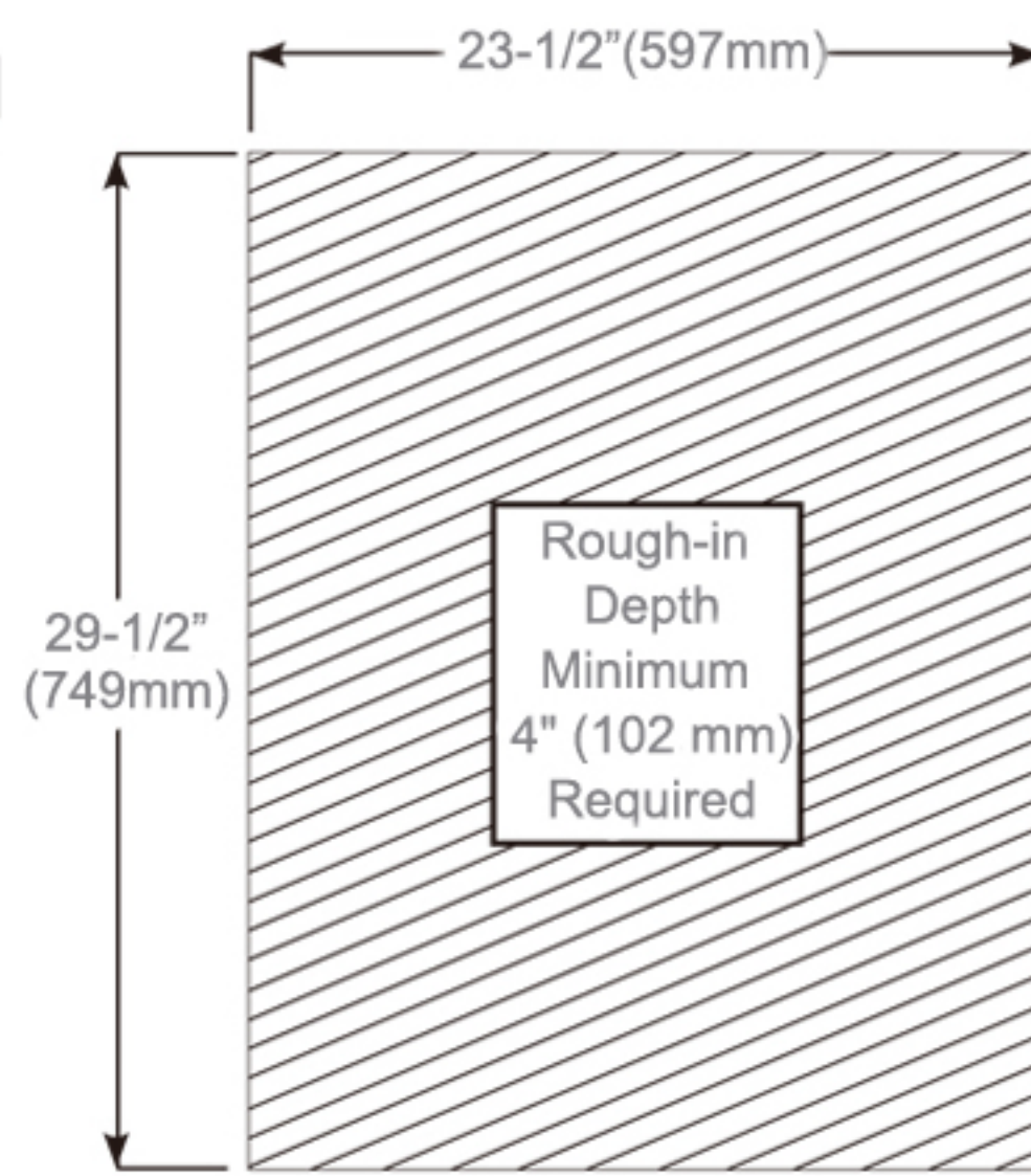
Rough-in Dimensions
