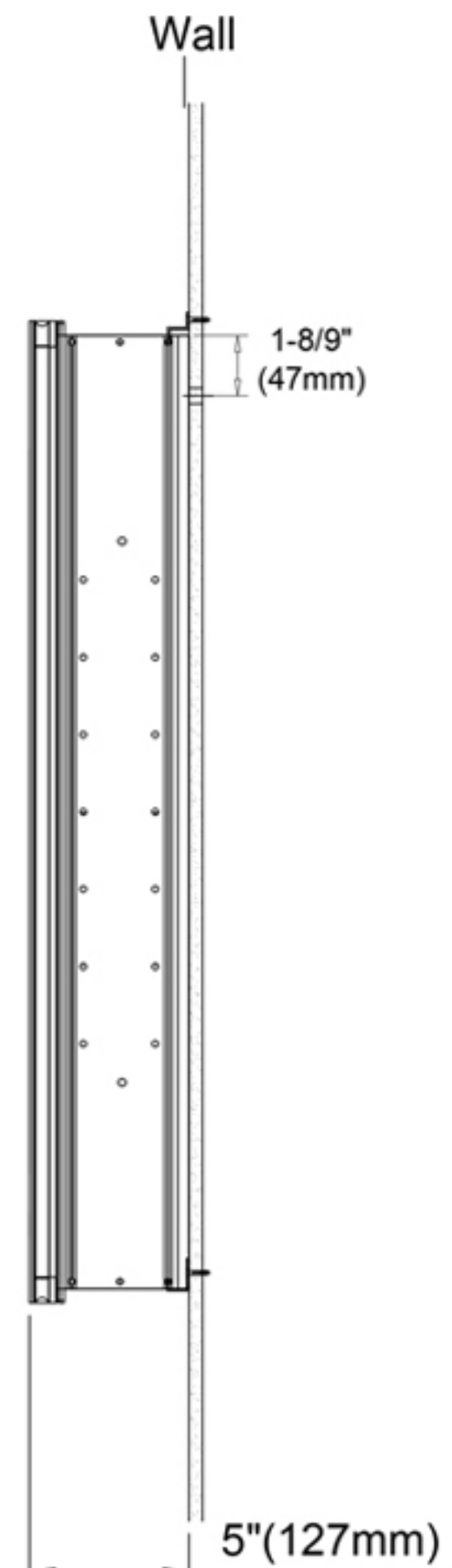
Surface Mount
