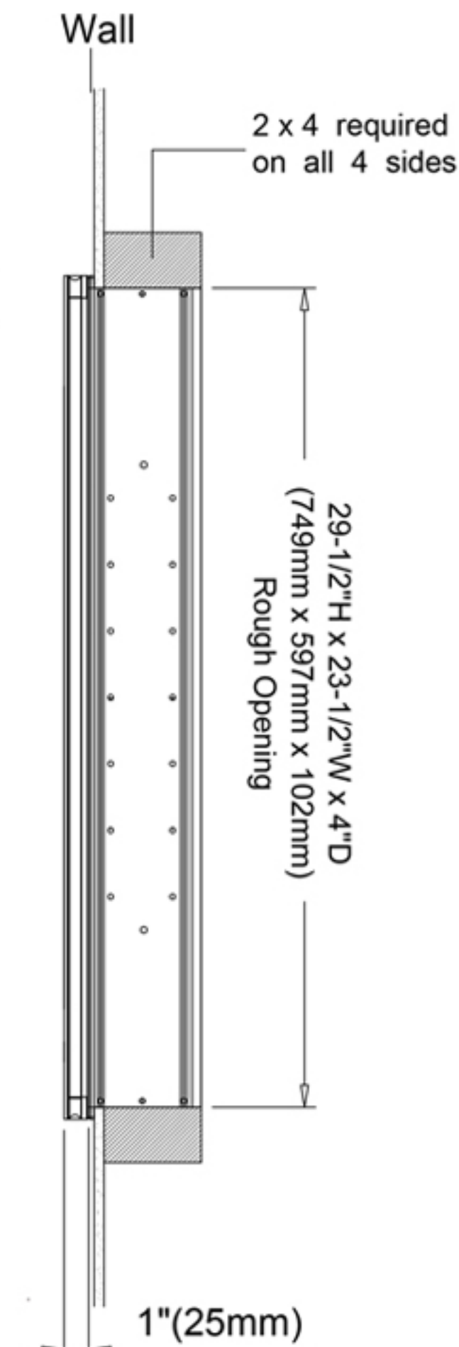
Recessed Mount
