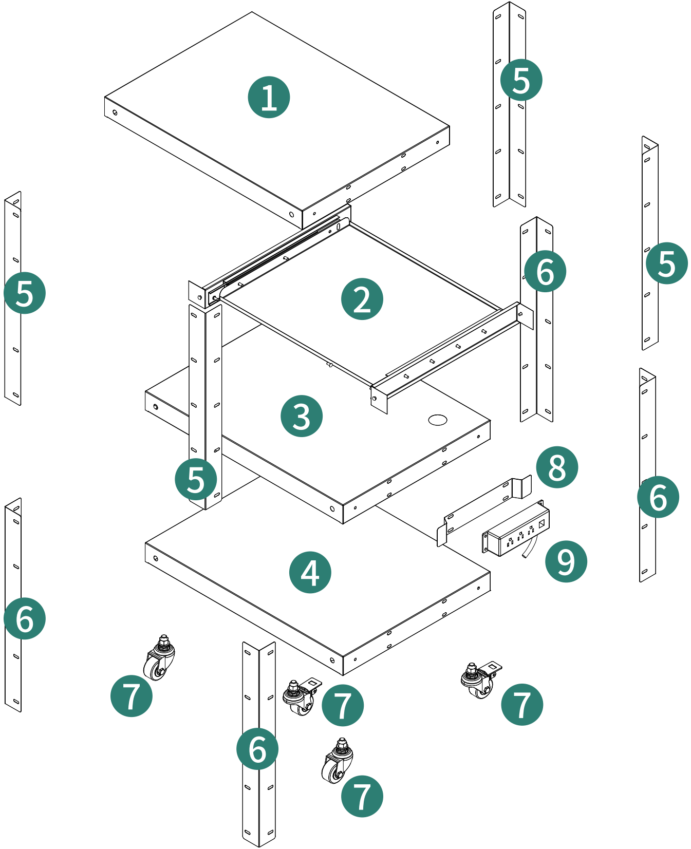
Explosion diagram
