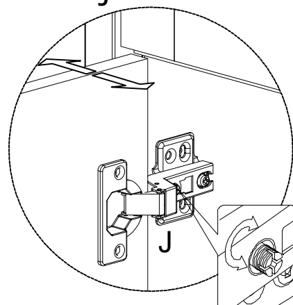
3.Left & Right Adjustment
