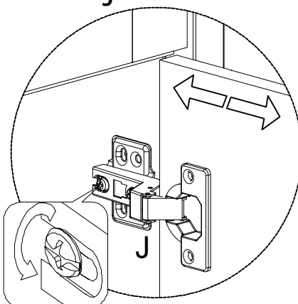
2.Forward & Back Adjustment
