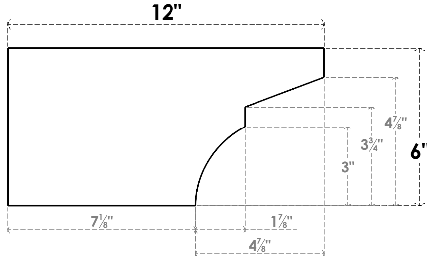
SIDE PROFILE
