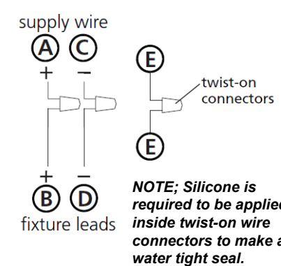
Drawing 3 – Post-Mount
