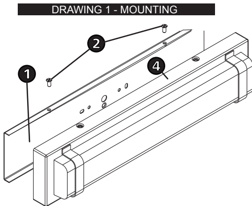
DRAWING 1 - MOUNTING
