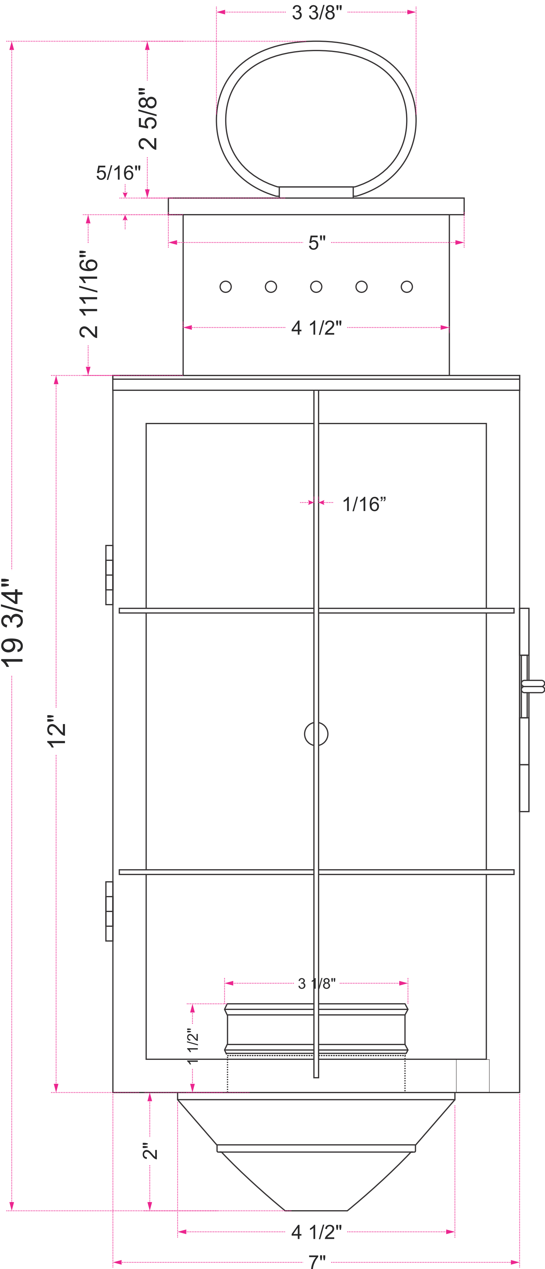
Front View
