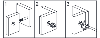
Cam Lock Fastening System
