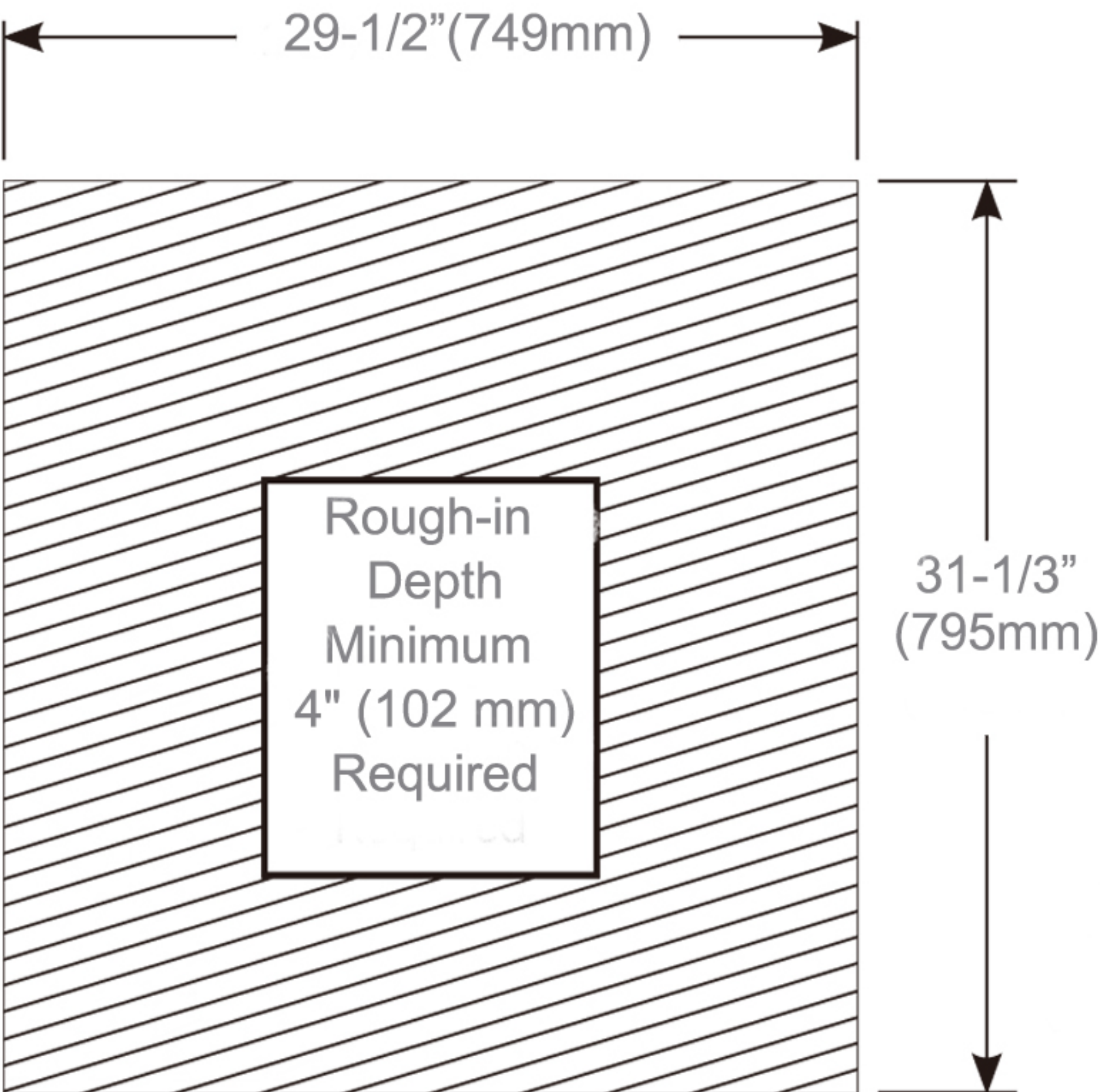
Rough-in Dimensions
