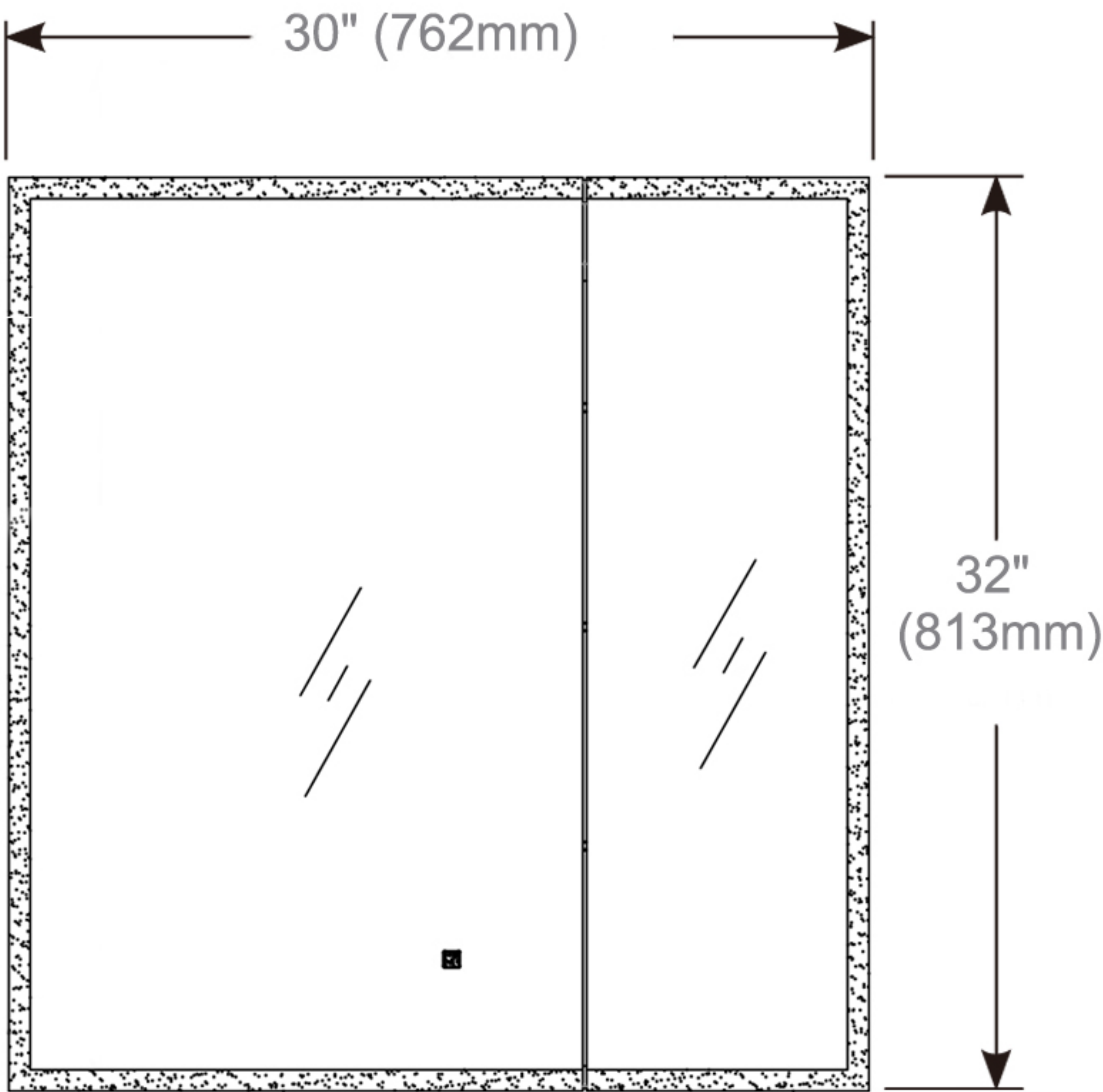
Cabinet Dimensions
