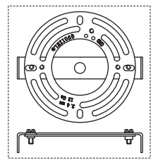
A Crossbar x 1
