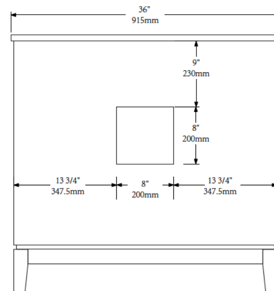
BACK VIEW
