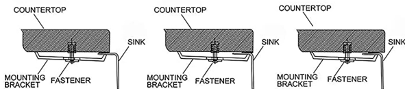
SPECIFICATION A: 1/4" REVEAL
