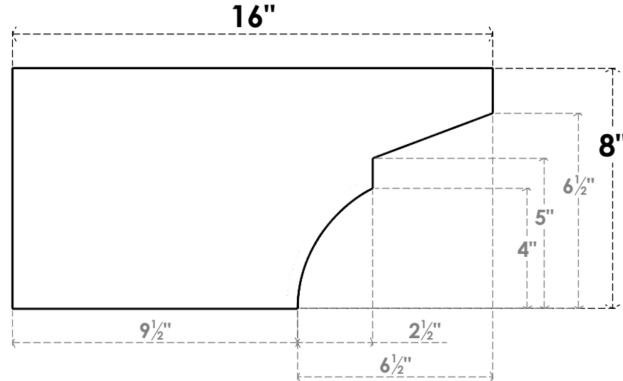
SIDE PROFILE
