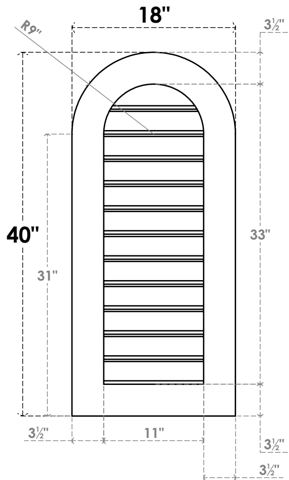
FRONT
