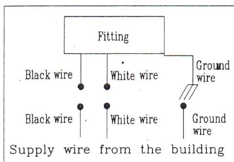
Circuit diagram 1
