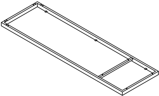
Top Frame
