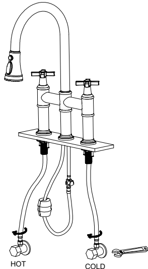
Hexagon Wrench
