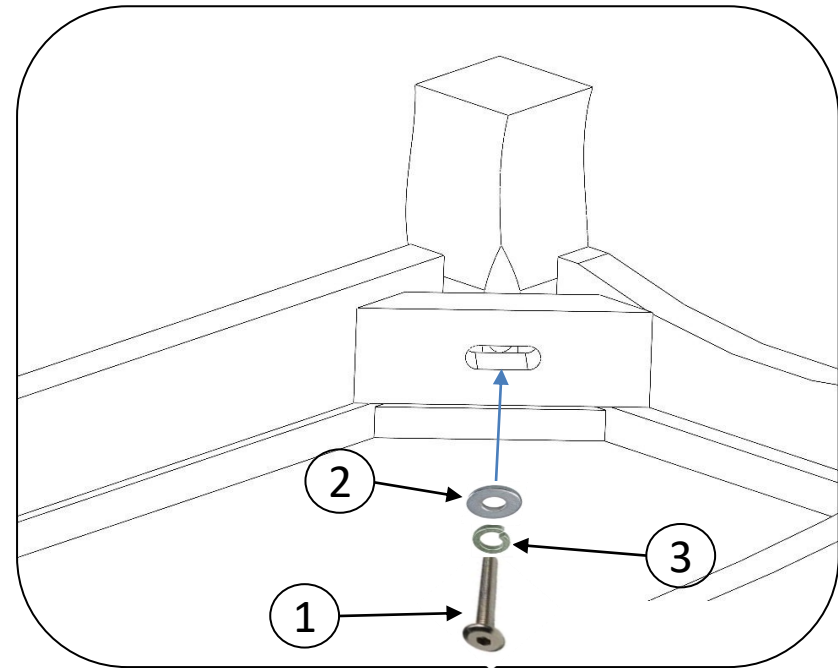
DETAIL X
