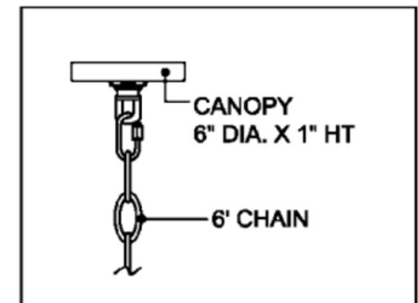
CANOPY DETAIL
