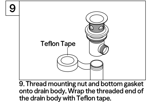
Teflon Tape
