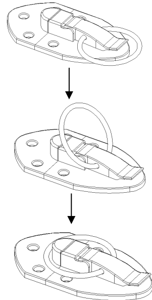
FIG-5 Buckle
