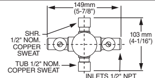
THREADED (STOPS) (R115SS)
