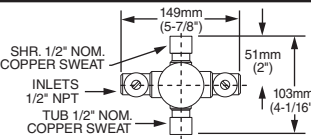
SWEAT (STOPS) (R110SS)
