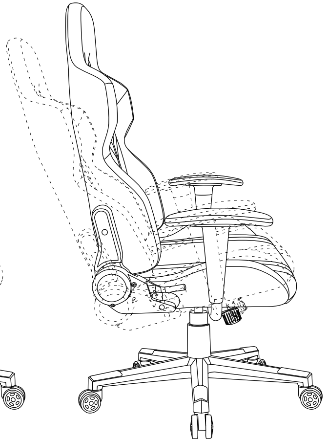
Counterclockwise rotation Rocking angle 0-30°
