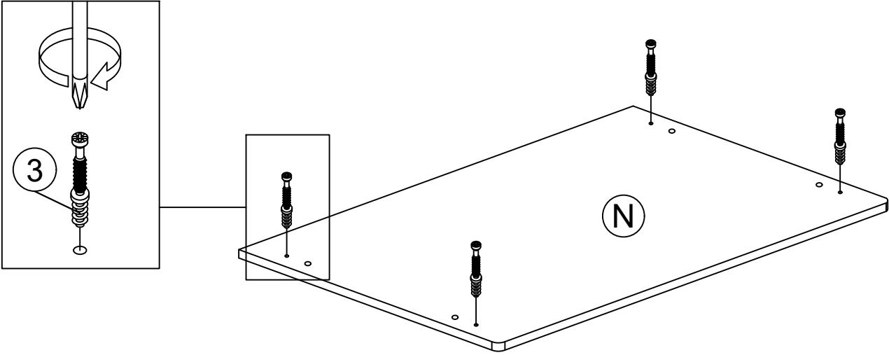
Bottom View
