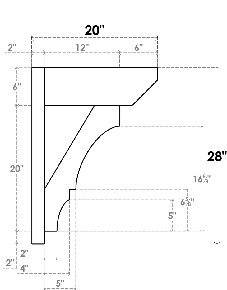
SIDE PROFILE
