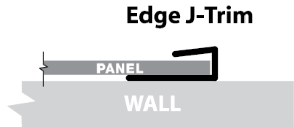
Top View - Cross Section End Point on Wall
