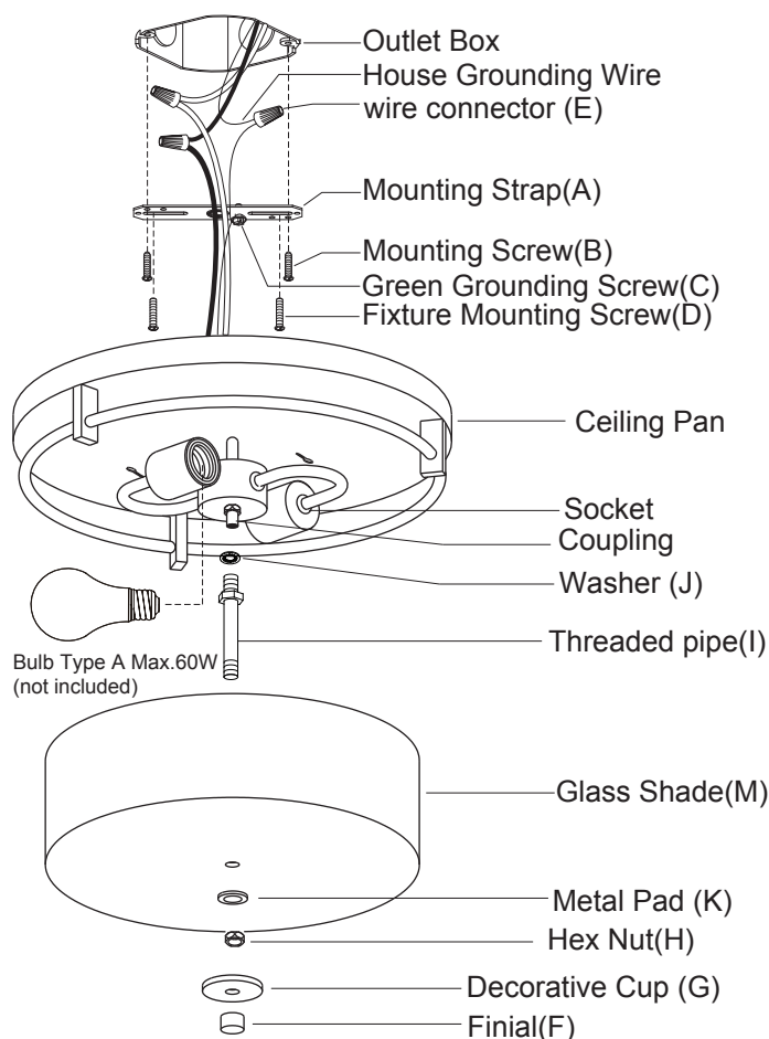
Threaded Pipe (I)
