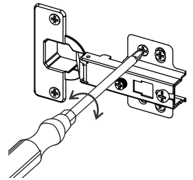
Front screws adjustment
