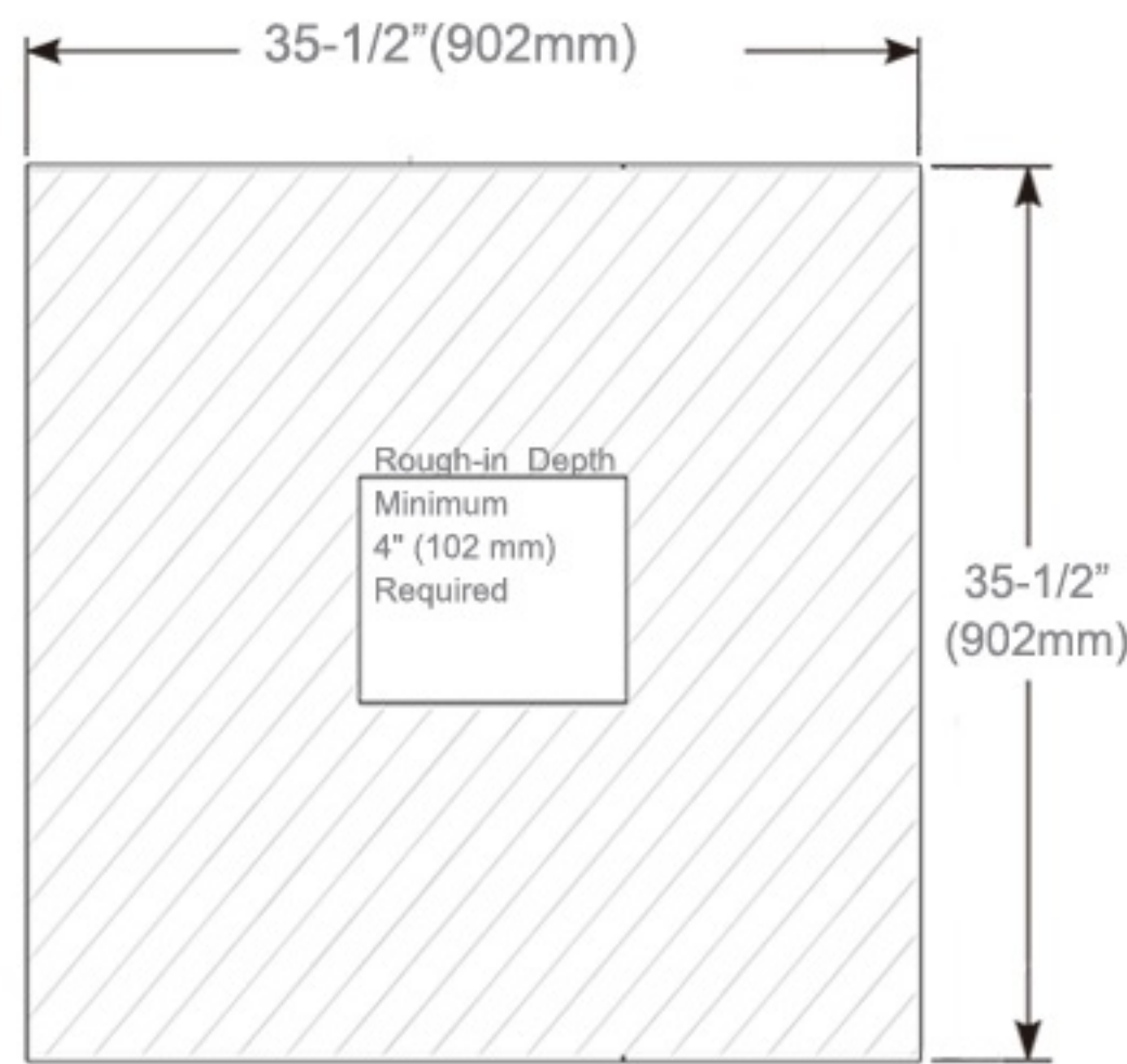
Rough-in Dimensions
