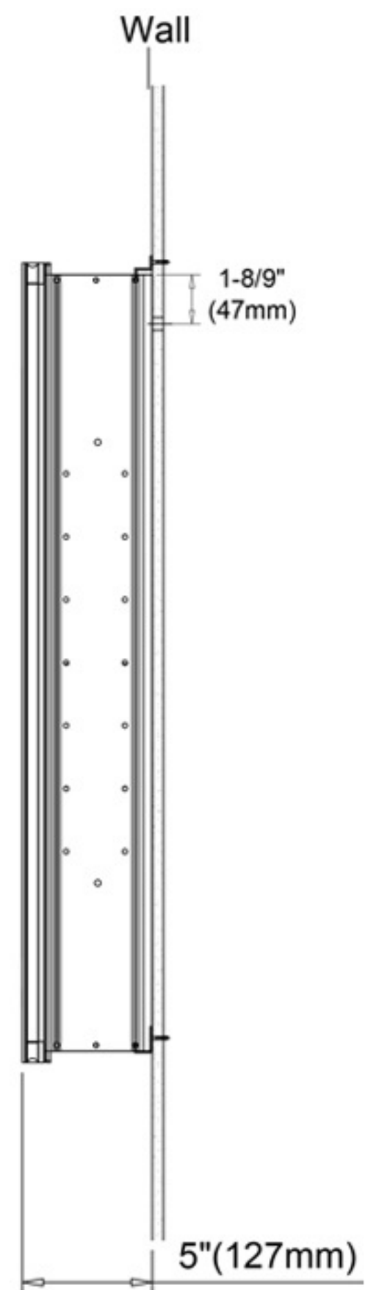
Surface Mount
