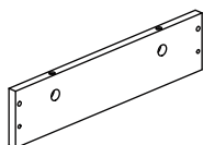
22 (335*80*12mm x2)
