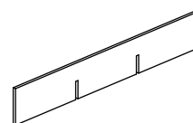
28 (399*62*5mm x4)
