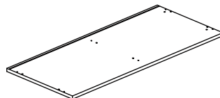
3 (916*400*15mm x1)
