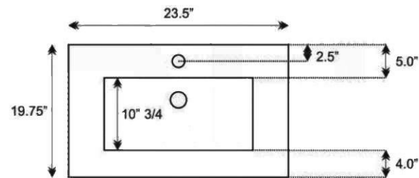
SINK CUT OUT OPENING 15.75"W x 10.75"D
