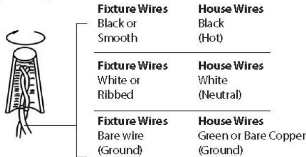
Fig.2 Wiring
