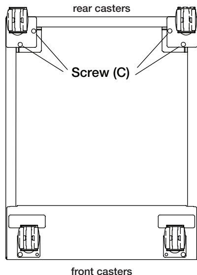
FIGURE 3: Complete assembly.
