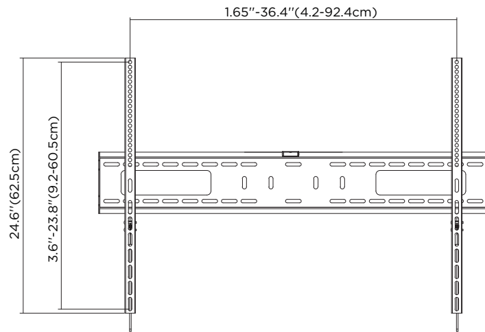
ORTHOGRAPHIC VIEW
