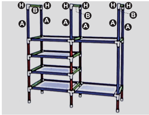
Step 4: Assemble 6× H, 3× B tube, and 6× A tube according to the picture.
