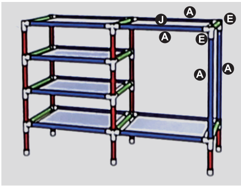
Step 3: Assemble 2× E, 4× tube A, 1×J and 1× tube B according to the picture.
