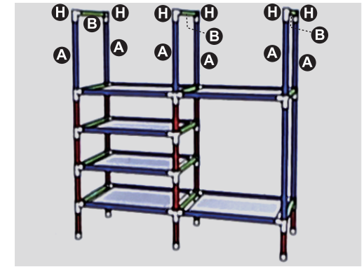
Step 4: Assemble 6× H, 3× B tube, and 6× A tube according to the picture.
